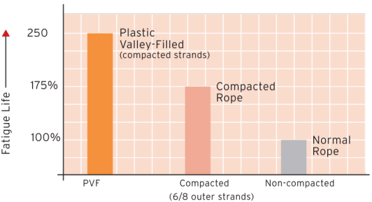
Comparison of service life (mining application)
