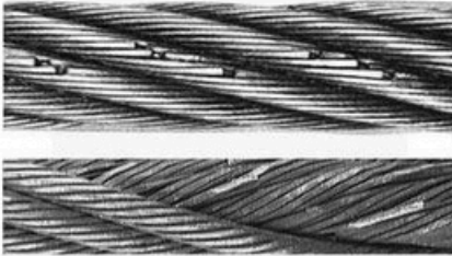
FATIGUE FAILURE
