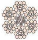
FLATTENED STRAND 6x22 (9/12-▲) & 6x25 (12/12-▲) FS Page # 87
