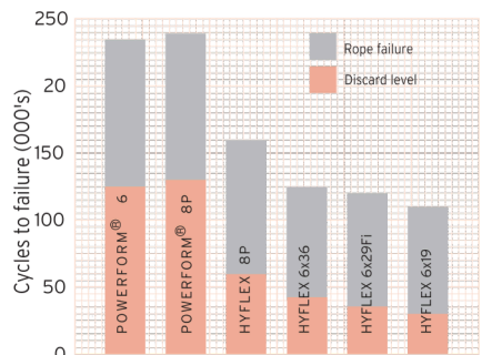
Comparison of bend fatigue illustration
